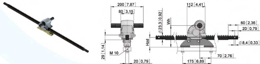
德国LOCK 桁架开窗齿轮齿条 LOCK truss rack and pinion
